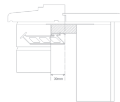
Sill detail
