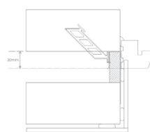
Staggered jamb
