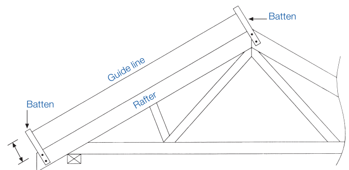
75mm + thickness of roof covering
